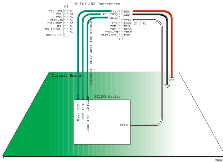
Figure 2-12 Verification of Configuration Data Only (Spartan, XC5200, XC4000)
