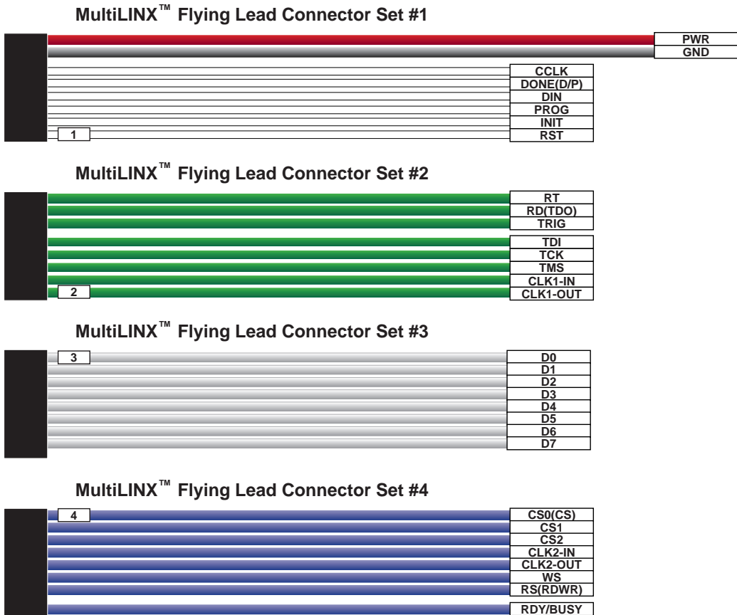
Figure 2-1 MultiLINX Flying Wires
