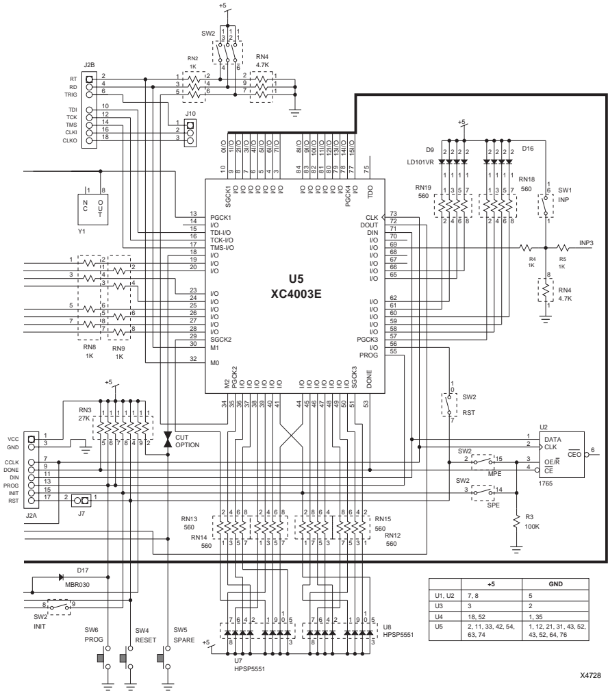
Figure 3-6 XC4003E Schematic
