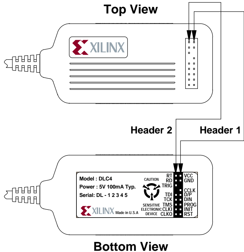
Figure 1-10 XChecker Cable
