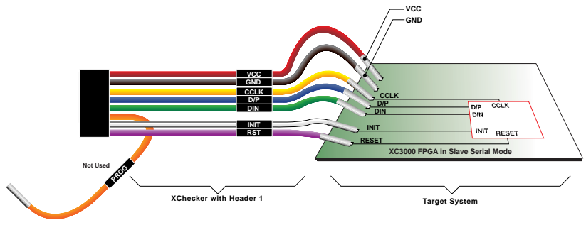
Figure 1-12 XChecker Connections to XC3000 Device
