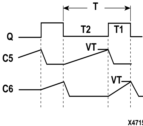
Figure 3-10 RC Network Waveforms
