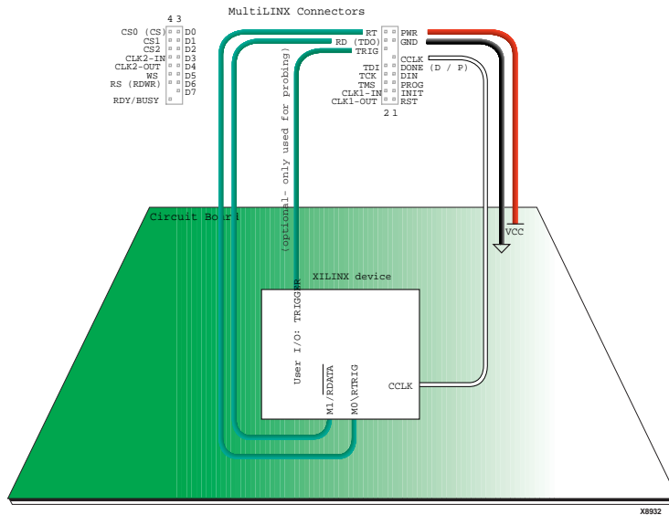
Figure 2-13 Verification of Configuration Data Only (XC3000)
