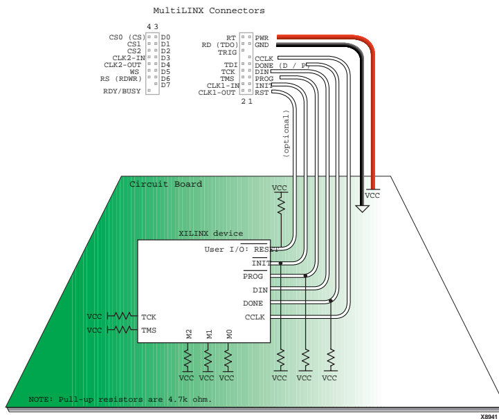
Figure 2-4 Slave Serial Mode (Virtex, Spartan, XC5200, XC4000)
