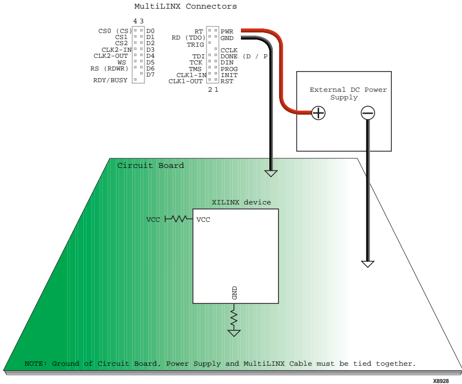
Figure 1-3 Optional External Power for the MultiLINX Cable
