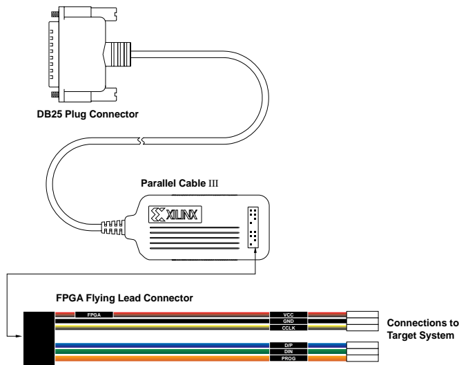
Figure 1-4 Parallel Cable III and FPGA Flying Leads
