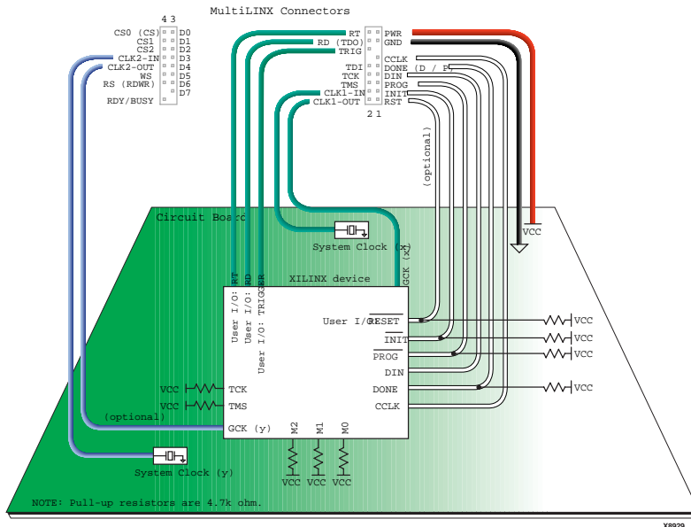
Figure 2-15 Slave Serial Mode (Spartan, XC5200, XC4000)
