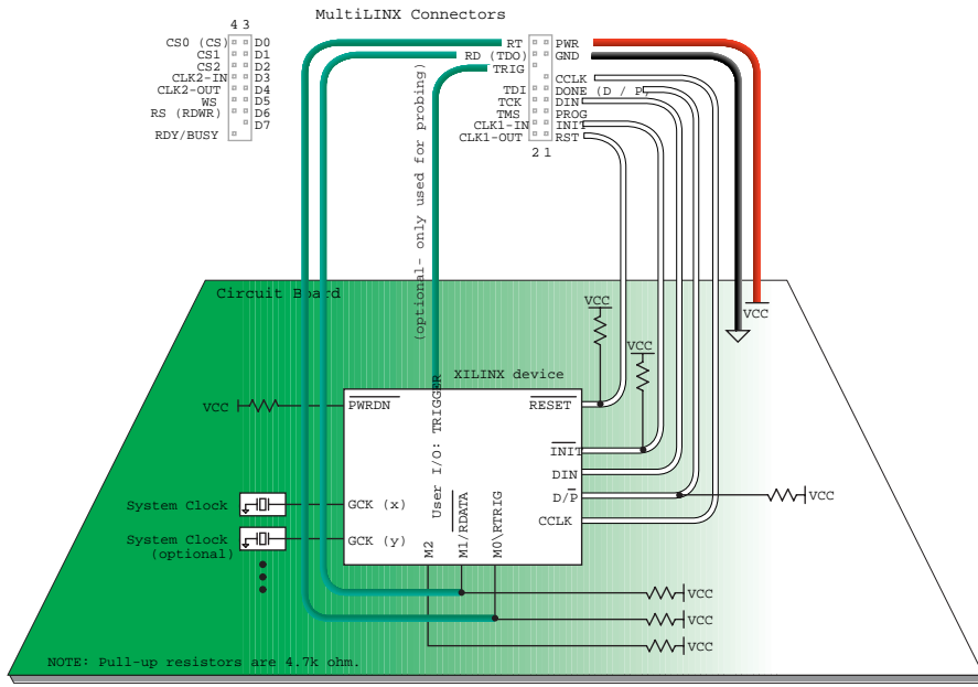
Figure 2-7 Slave Serial Mode (XC3000)
