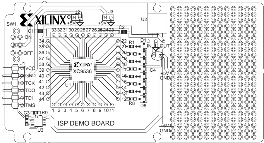
Figure 4-2 CPLD ISP Demonstration Board
