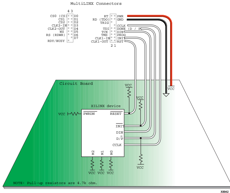
Figure 2-3 Slave Serial Mode (XC3000)
