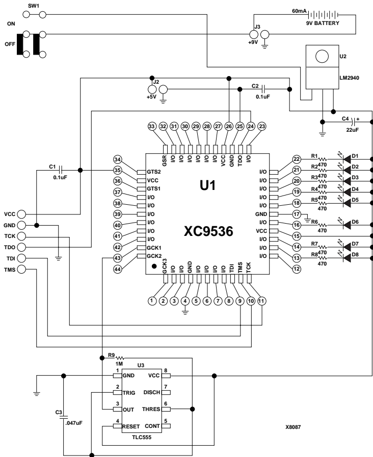
Figure 4-1 XC9536 Device Schematic
