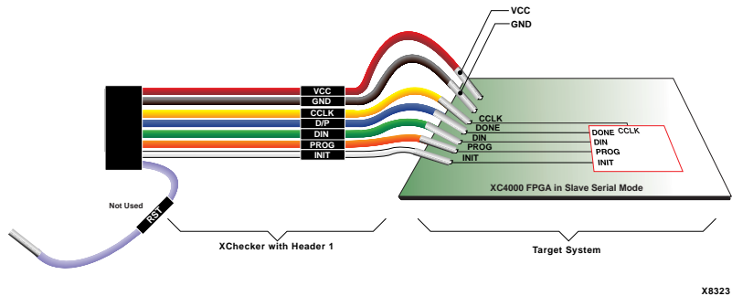
Figure 1-11 XChecker Connections to XC4000 Device
