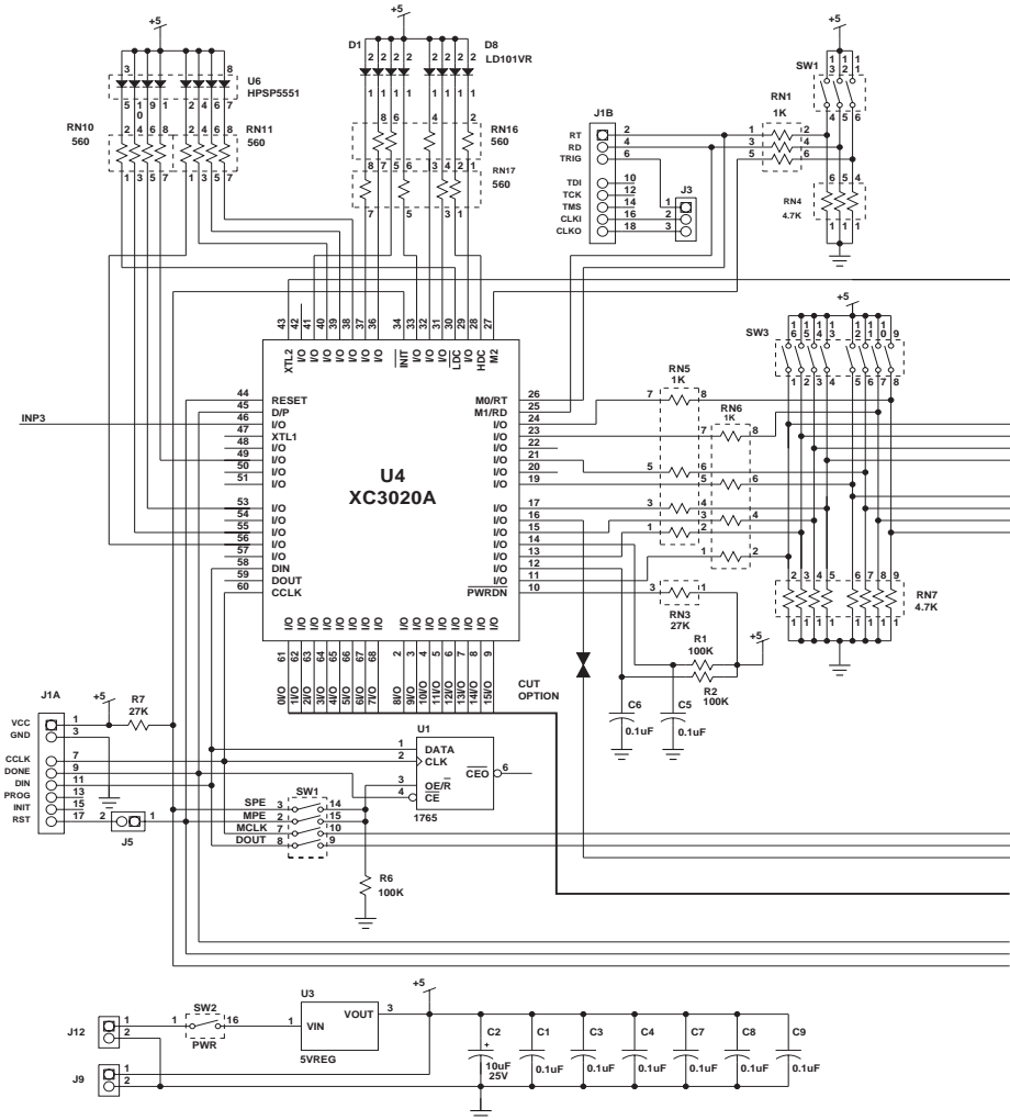
Figure 3-7 XC3020A Schematic
